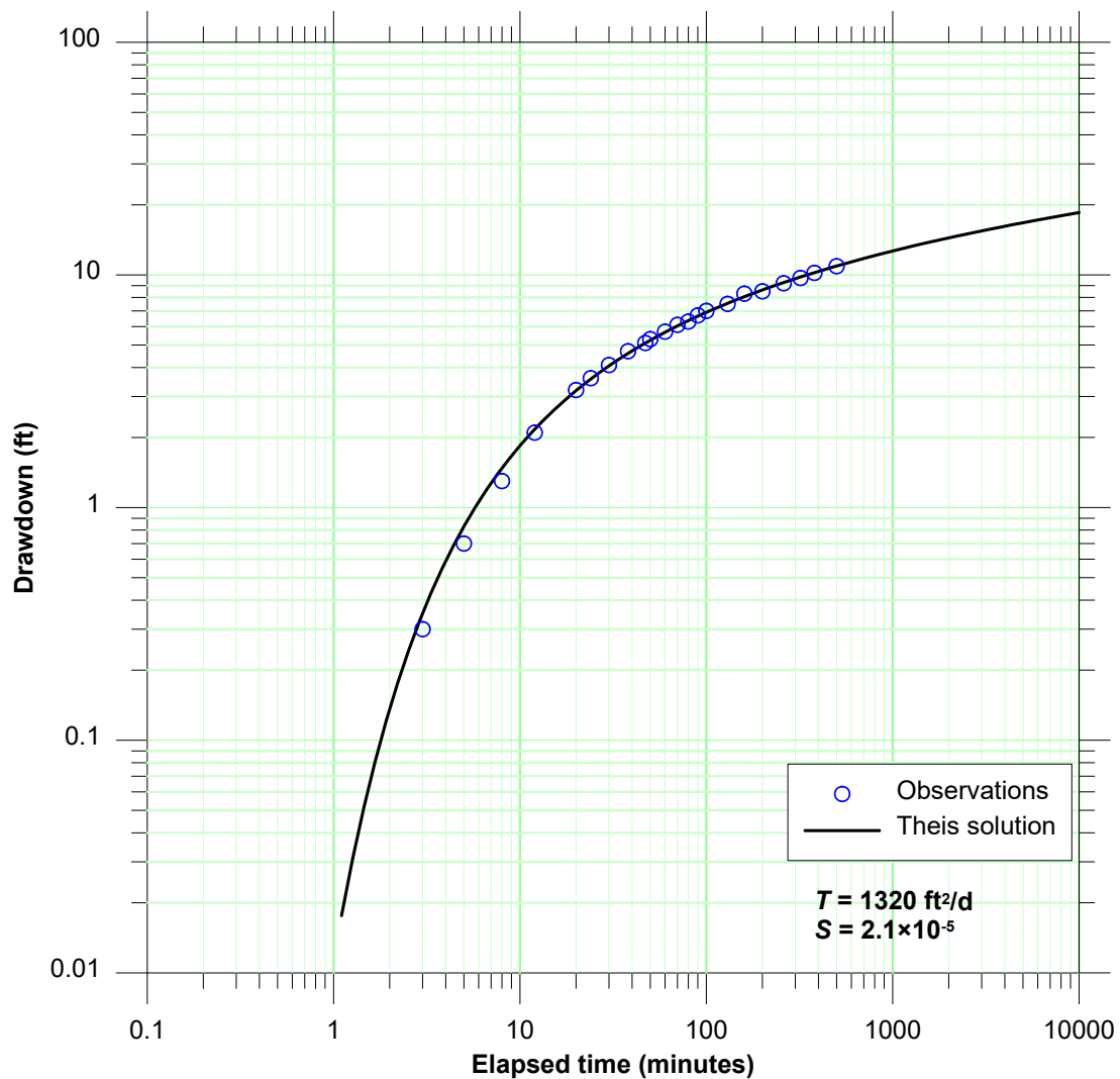
Figure 6. Match of the drawdowns with the Theis solution
