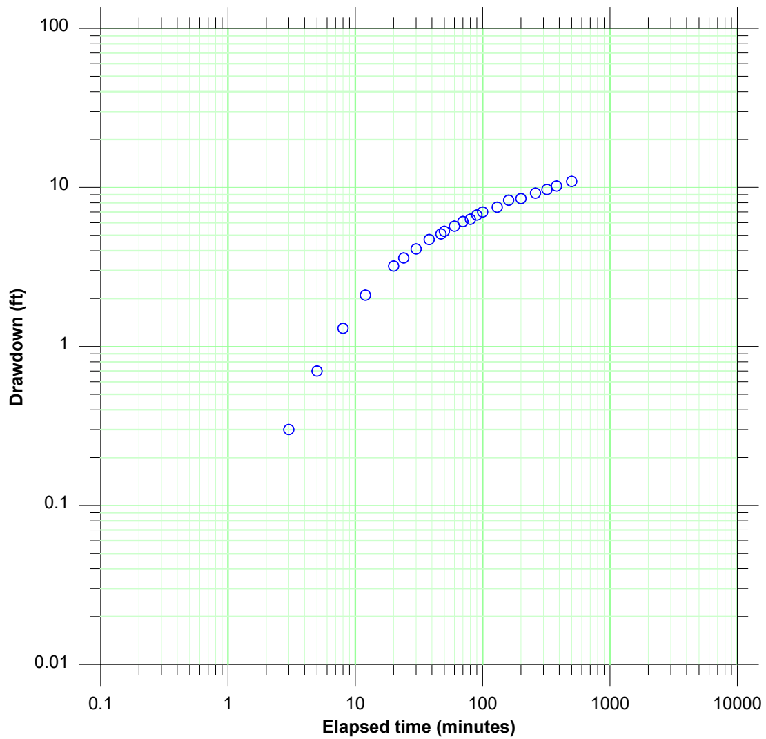
Figure 4. Drawdowns for Gridley observation Well No. 1 Data from Walton (1970)
