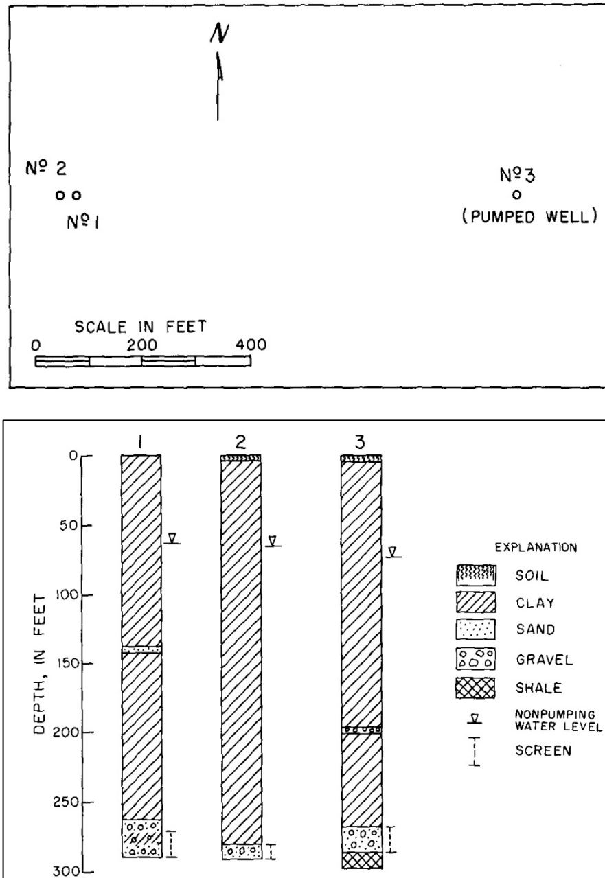
Figure 3. Gridley, Illinois pumping test layout
