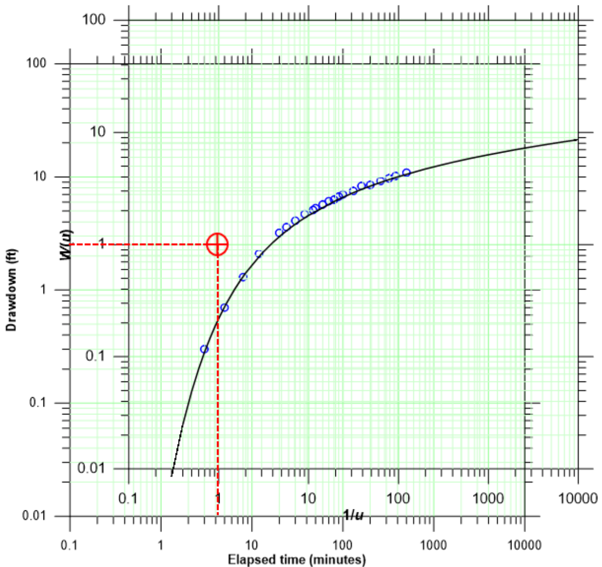
Figure 5. Gridley example, Theis type-curve match
