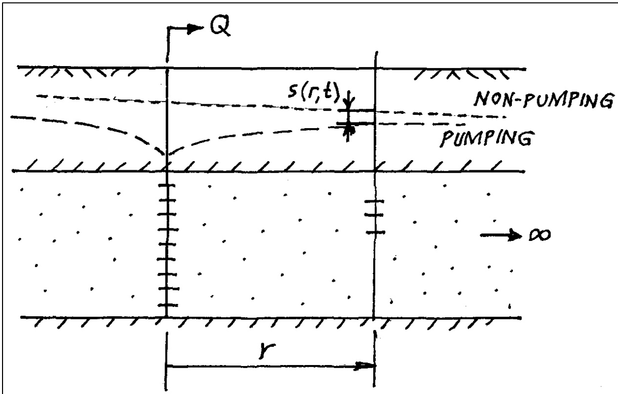
Figure 1. Conceptual model of the Theis solution
