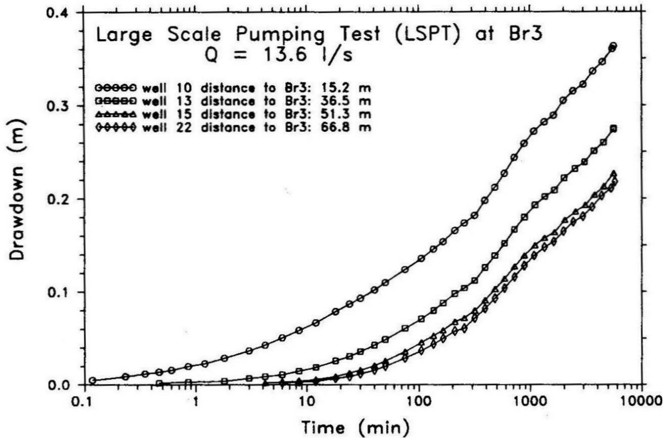
Figure 31. Drawdown data for selected observation wells Reproduced from Schad and Teutsch (1994)
