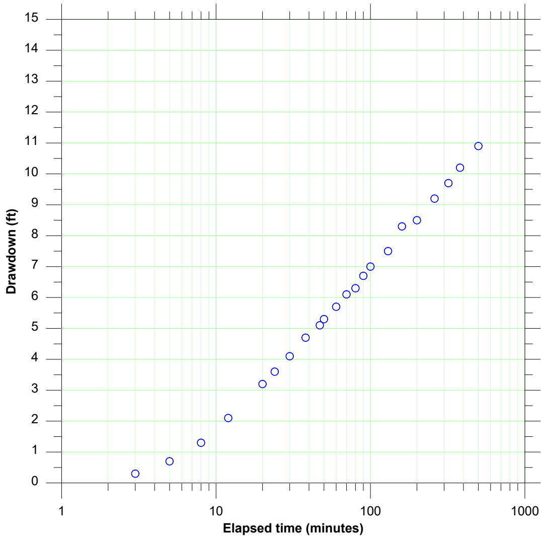
Figure 8. Drawdowns for Gridley observation Well #1 Data from Walton (1970)
