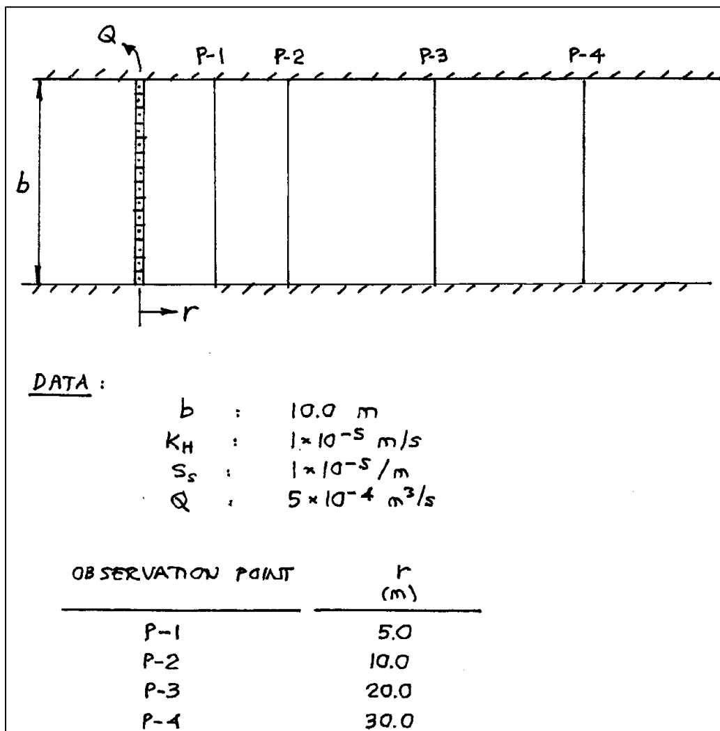
Figure 24. Example pumping test with multiple observation wells
