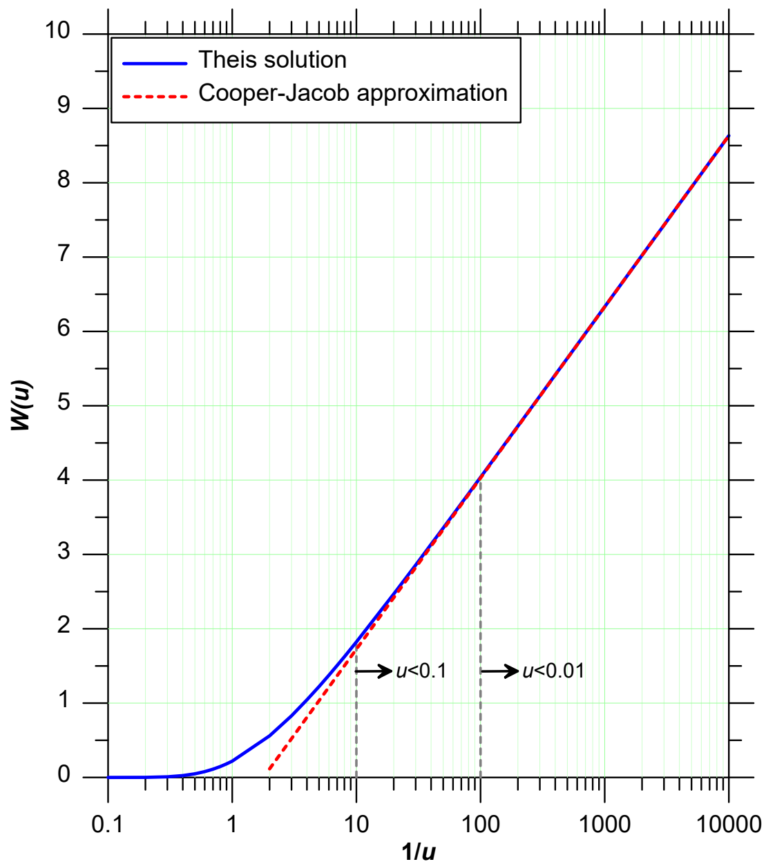
Figure 7. Cooper-Jacob approximation of the Theis well function
